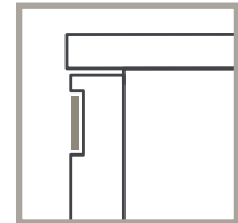
BLEND AD INCASSO ANTA CON MANIGLIA INCASSATA RECESSED BLEND / DOOR WITH RECESSED HANDLE
